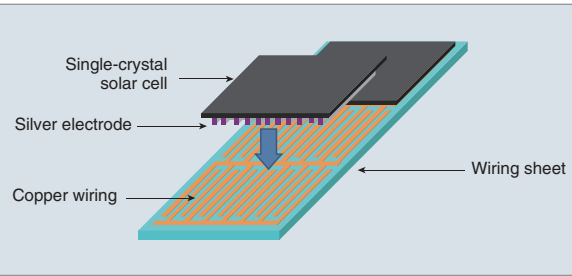
In a Blacksolar PV cell, the silver electrode and copper wiring are directly connected, and the line width is thicker, reducing the loss of generated power (schematic diagram)
