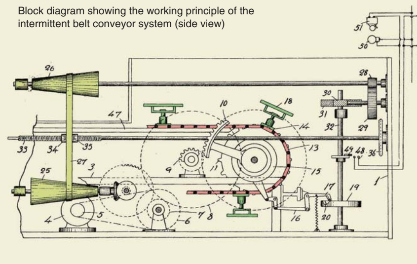
No. 18 is the work platform that alternately starts and stops with the movement of the conveyor belt. The action of pulleys 25 and 26 is a mechanism that enables the pause duration to be adjusted.
