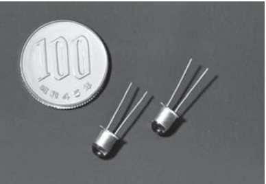
The GLE-50G gallium arsenide double LED emitted visible green light and near-infrared light simultaneously
