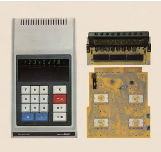
The QT-8D, the world's first LSI calculator (left) and its substrate fitted with MOS LSI
