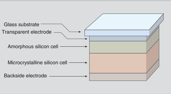
Crystalline thin-film tandem solar cells use a dual-layer cell structure to generate electricity from sunlight over a wide range of wavelengths (schematic diagram)
